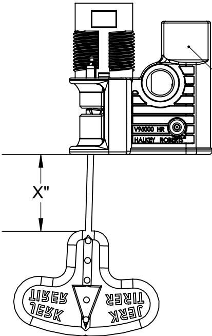
INFLATOR ASSEMBLY
